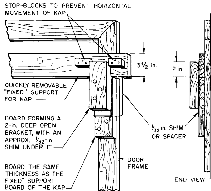
Fig. 19. Quick-removal bracket for KAP.
