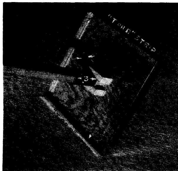
Fig. 14. Plywood Piston with Sheetmetal Sealing Strips Attached.
