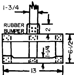
Fig. 15. Piston Rod Handle Made of \frac{3}{4} x 1\frac{3}{4} -in. Boards.
