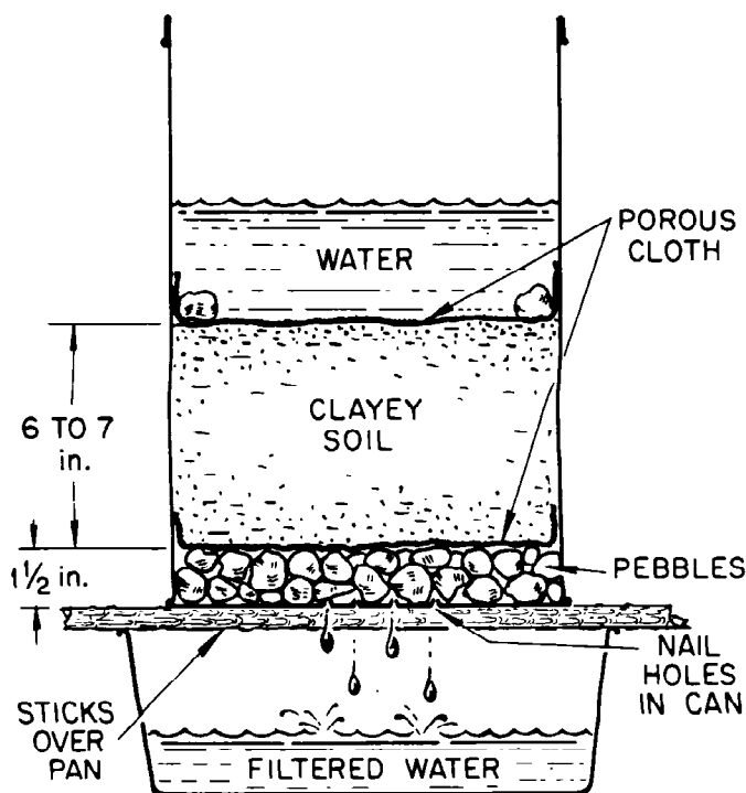
EXPEDIENT FILTRATION
