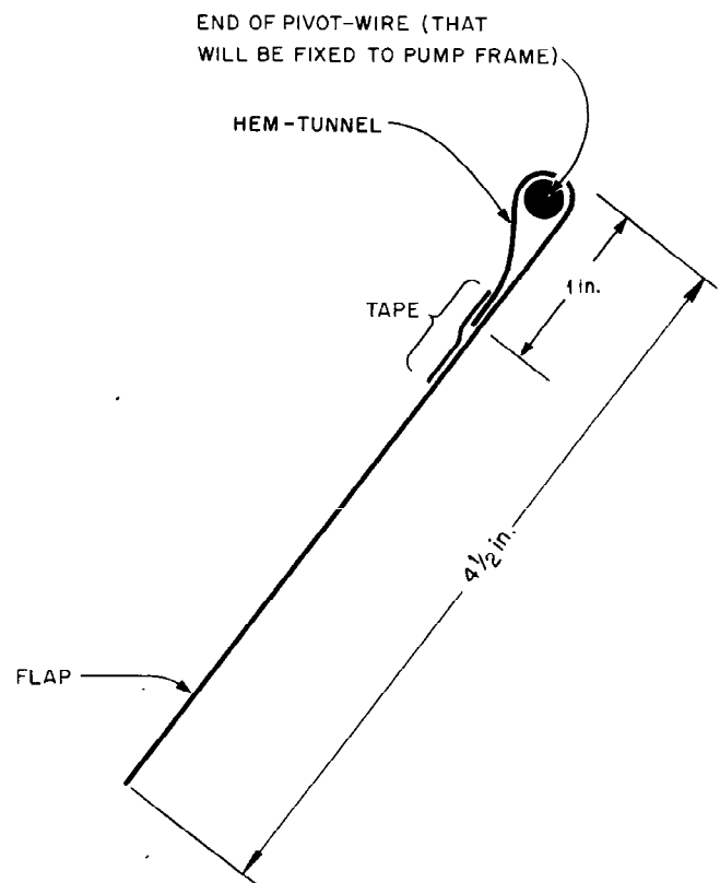
Fig. 7. End view.
