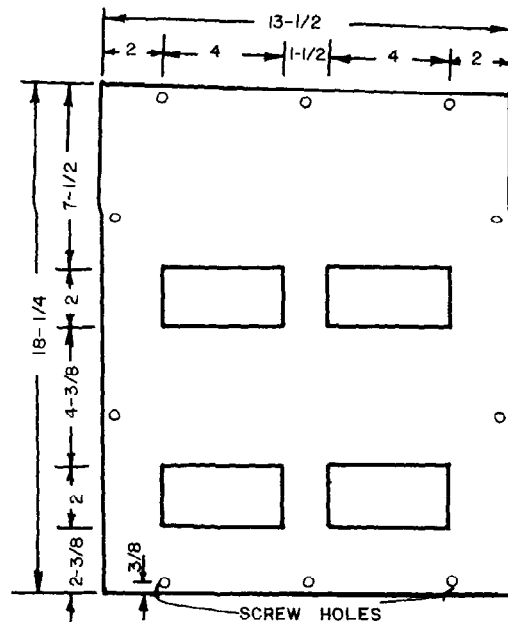
Fig. 8. Back End. Only the plywood is shown.
