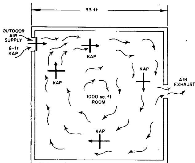
Fig. 16. The use of air-distribution KAPs.
